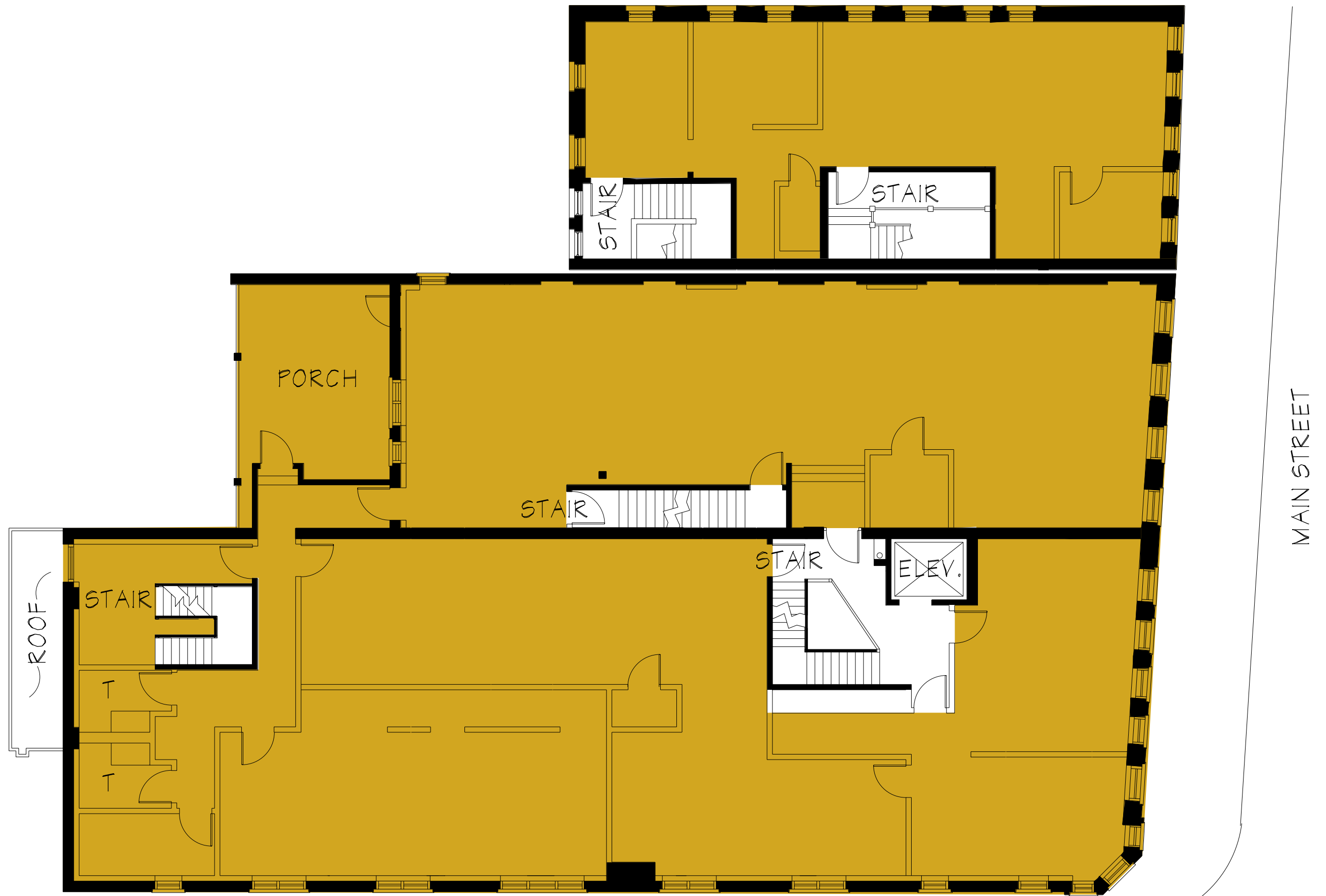
•THIRD FLOOR PLAN. AUGUST 2000
