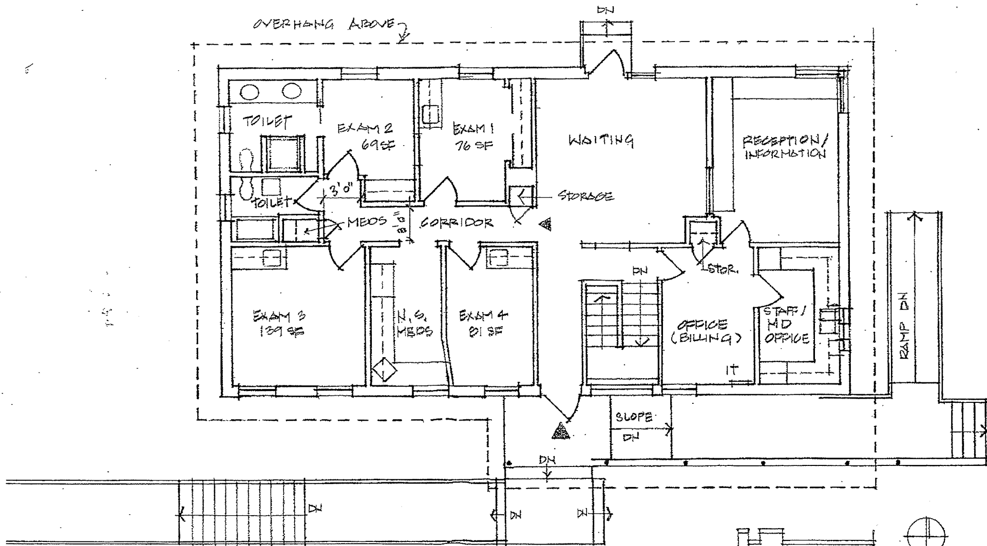
UPPER LEVEL EXISTING CONDITIONS PLAN
