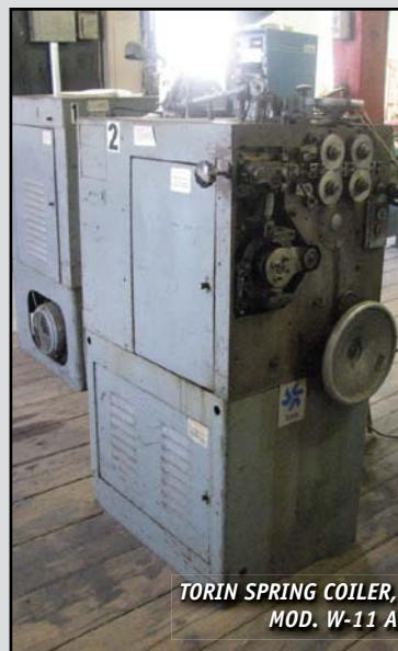
BHS-TORIN CNC SPRING COILER
