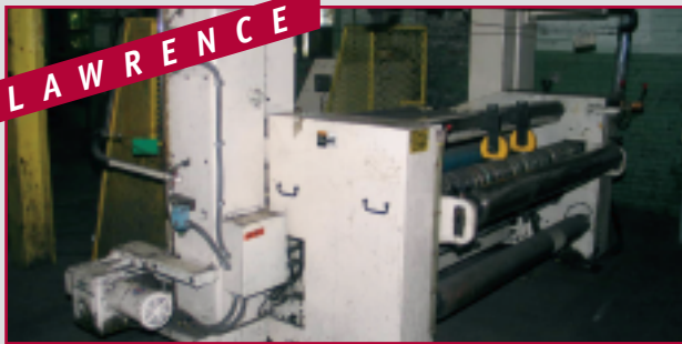
WEBCO SLITTER-REWINDER
