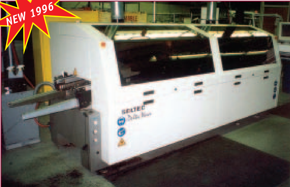
1996 DOVER SOLTEC "DELTA WAVE" WAVE SOLDERING MACHINE MOD. 6622C
